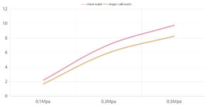
GPK012/AC flow rate L/MIN
